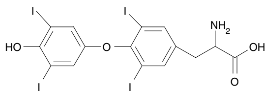
Figure 1. Molecular formula of thyroxine (3,3',5,5'-tetraiodothyronine).
