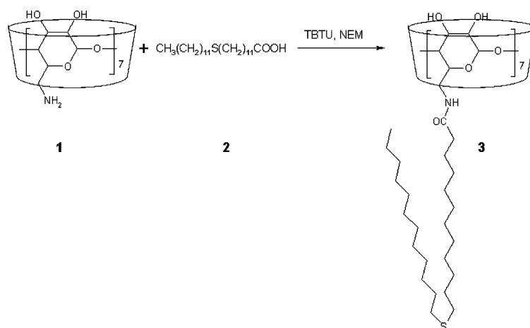
Figure 2. Synthesis of Heptakis{6-deoxy-6-[12-(thiododecyl)undecanamido]}- \beta -cyclodextrin, TBTU: O -Benzotriazol-1-yl- N,N,N',N' -tetramethyluronium tetrafluoroborate and NEM: N -ethylmorpholine.
