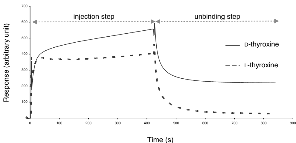
Figure 3. Binding sensograms of D- and L-thyroxine, values are expressed in arbitrary units and normalized to 0 at the beginning of the injection.
