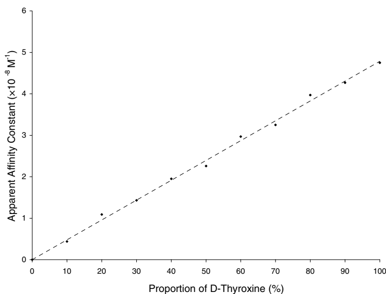
Figure 5. apparent affinity constants measured for varying proportions of D- and L-thyroxine.
