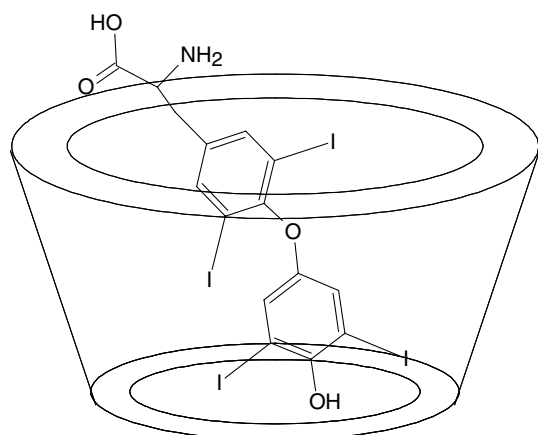
Figure 4. Schematic representation of the inclusion complex of thyroxine in the cyclodextrin cavity.
